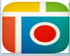
Show Me
